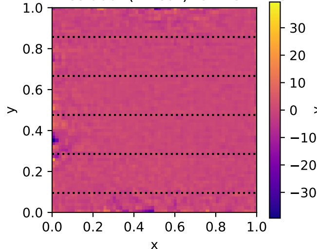
PDE Residual (Linear) for BC k=20
