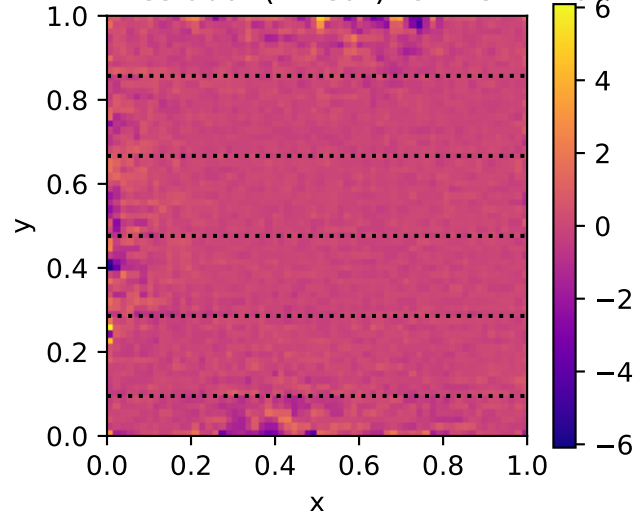
PDE Residual (Linear) for BC k=20
