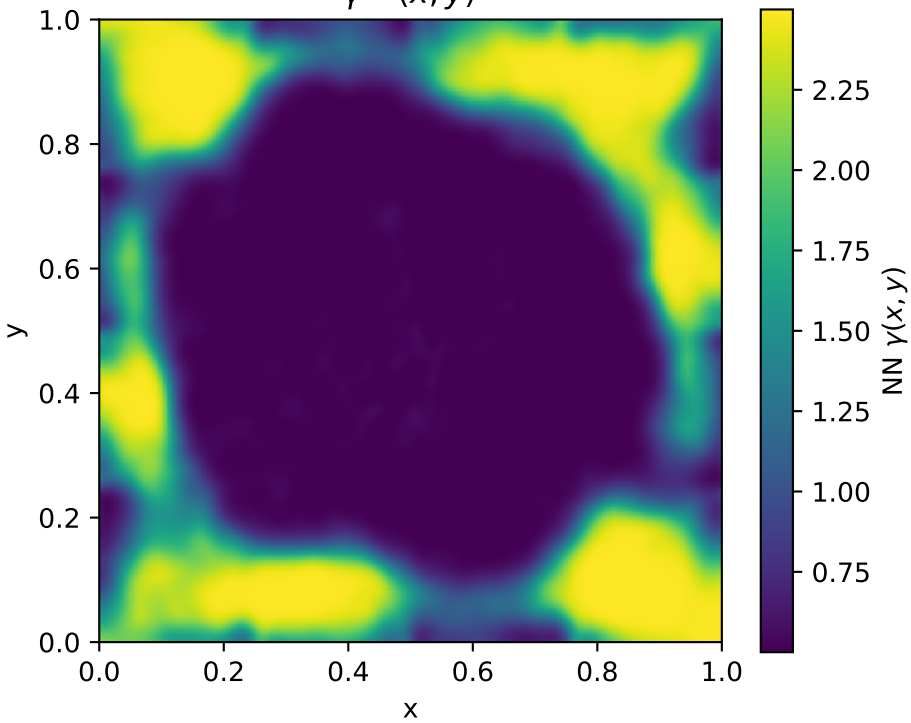
\gamma^{NN}(x, y)
