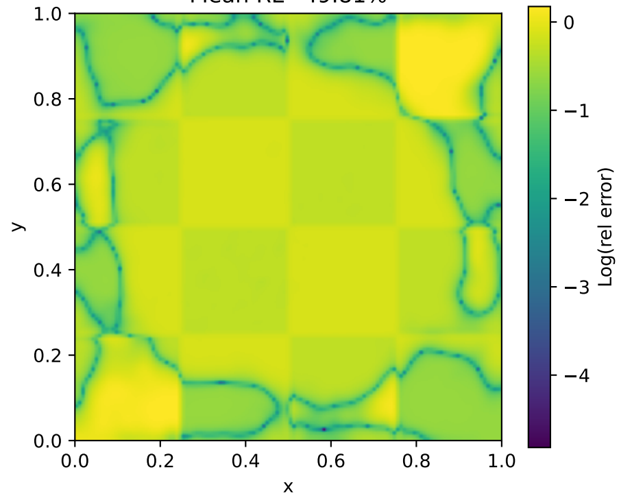
Mean RE=49.81%
