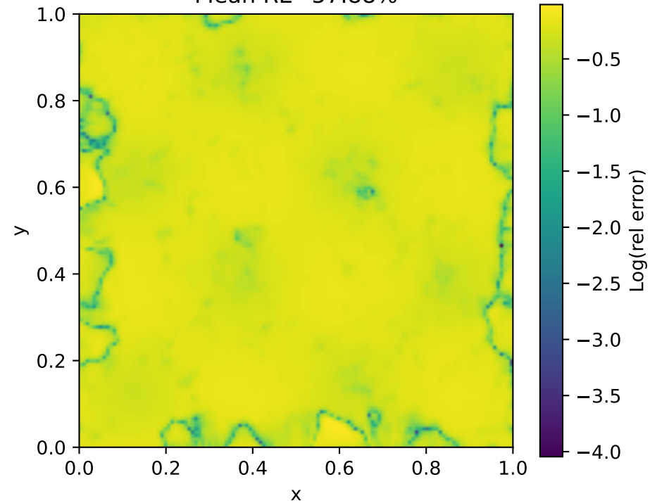
Mean RE=57.88%
