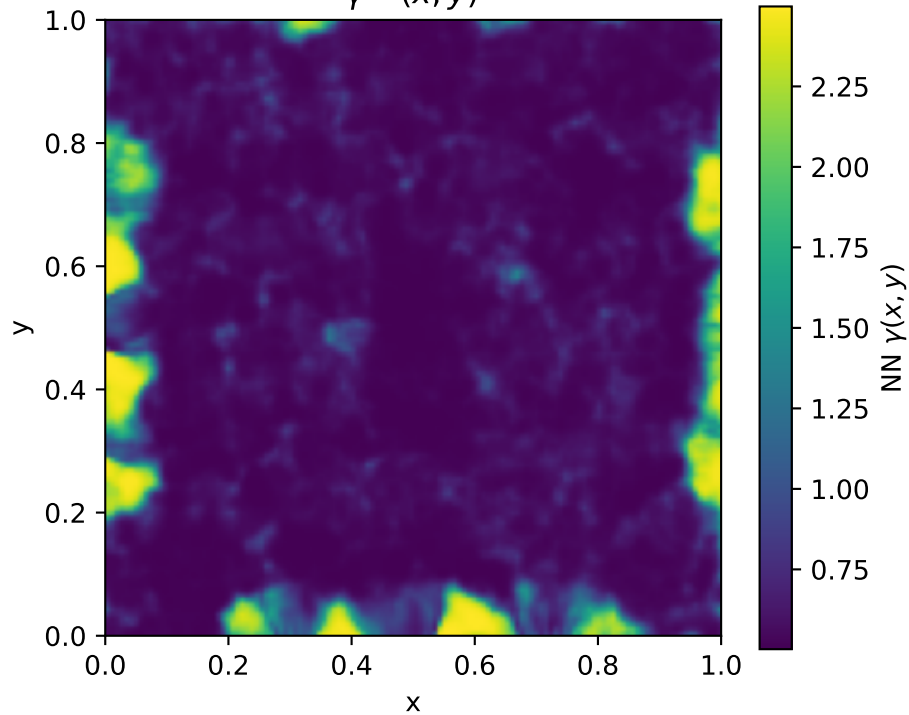
\gamma^{NN}(x, y)
