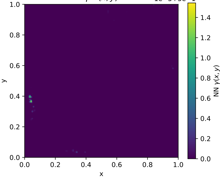
\gamma^{NN}(x, y)
