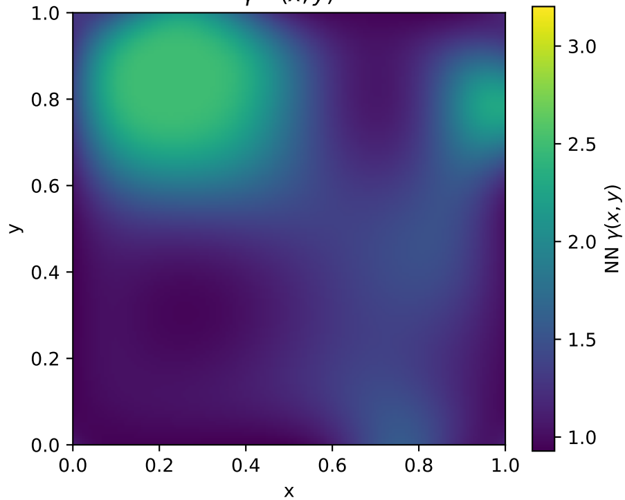
\gamma^{NN}(x, y)
