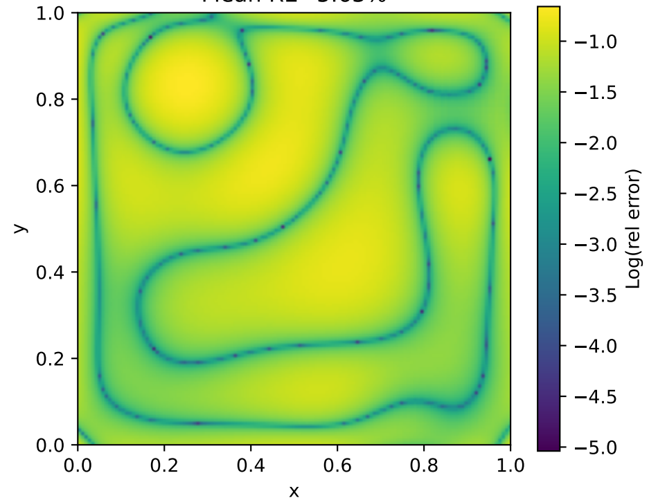
Mean RE=5.63%
