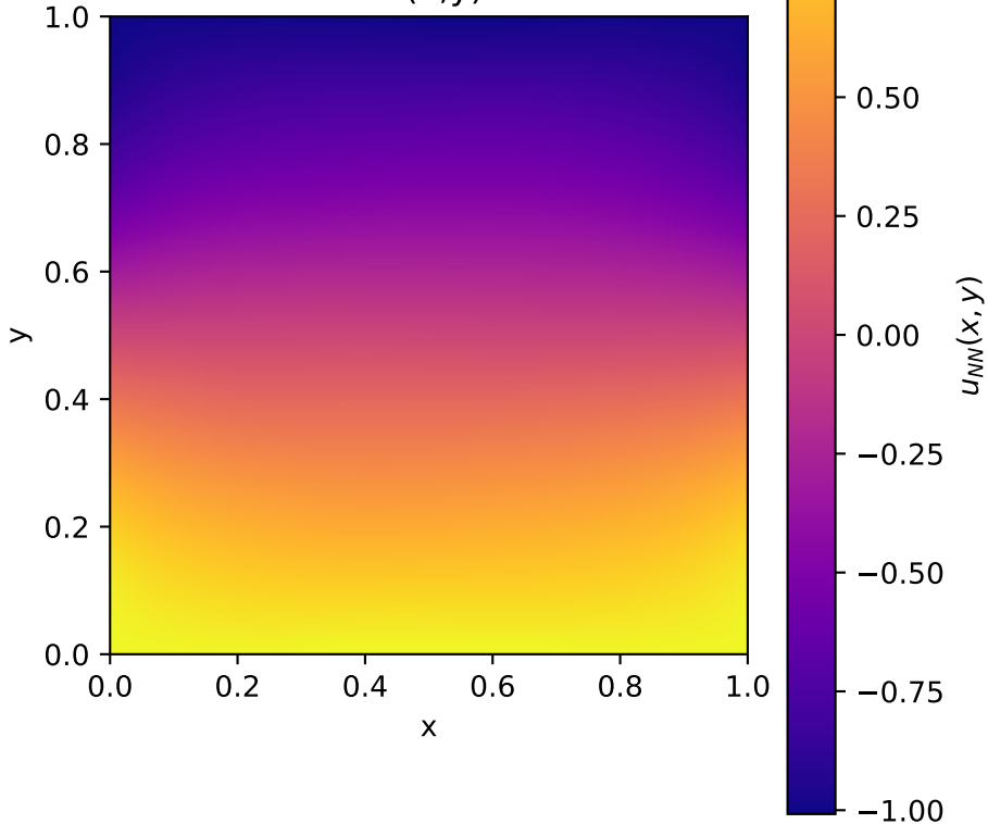
Induced u(x,y) for k=0
