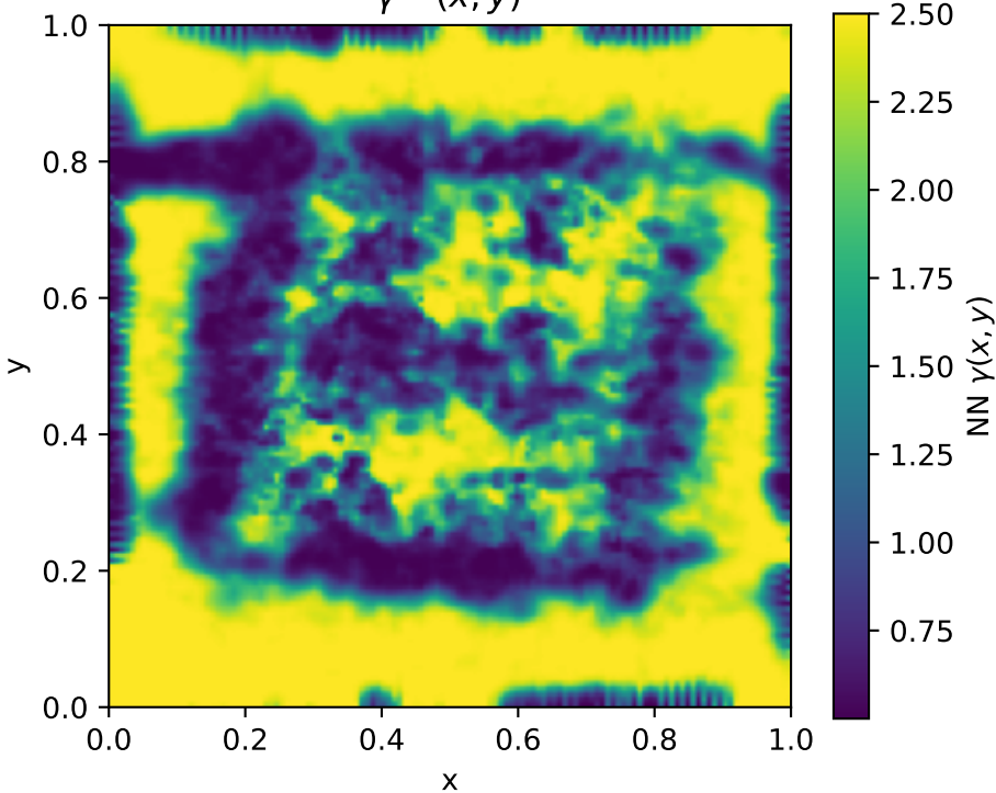
\gamma^{NN}(x, y)
