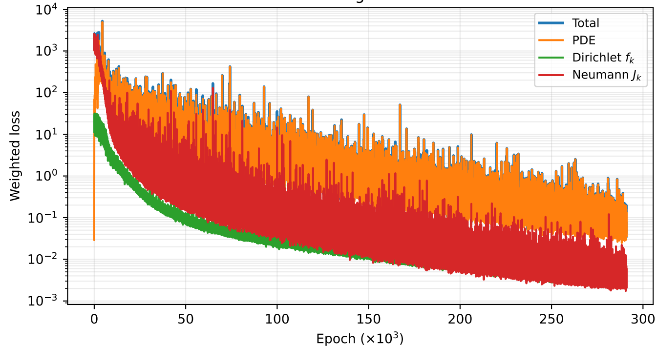
Training losses
