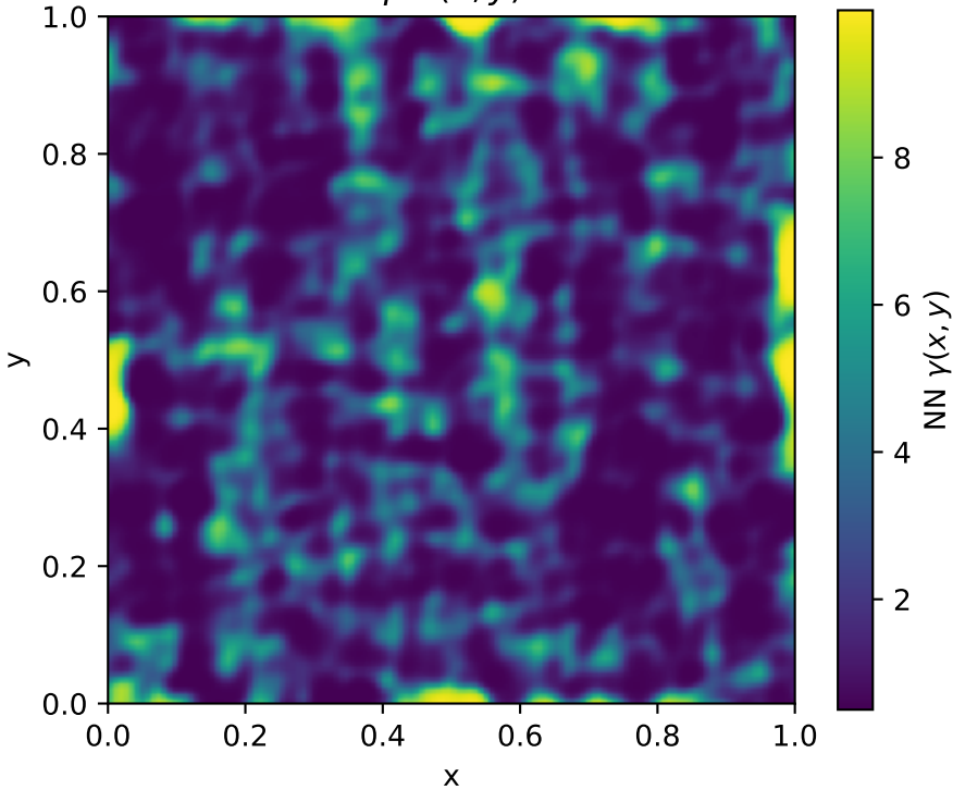
\gamma^{NN}(x, y)
