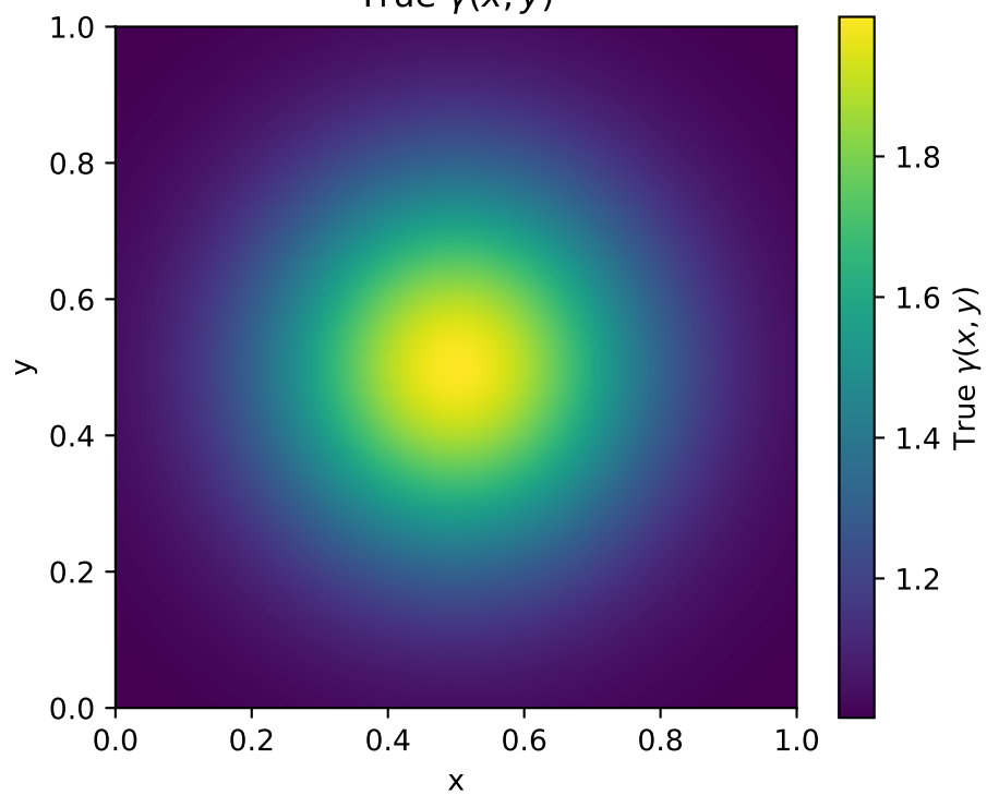
True \gamma(x, y)
