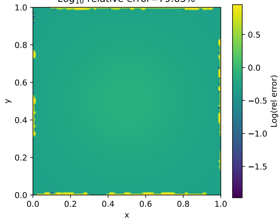
\text{Log}_{10} relative error=79.63%
