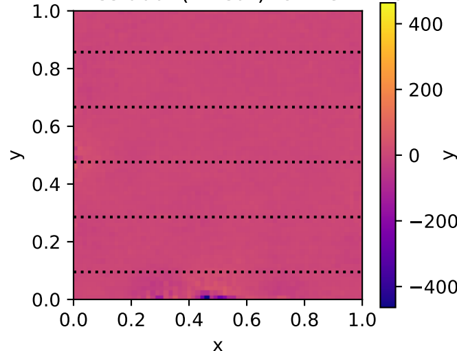
PDE Residual (Linear) for BC k=49
