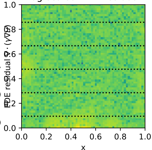
k=49 Log-scaled PDE Residual
