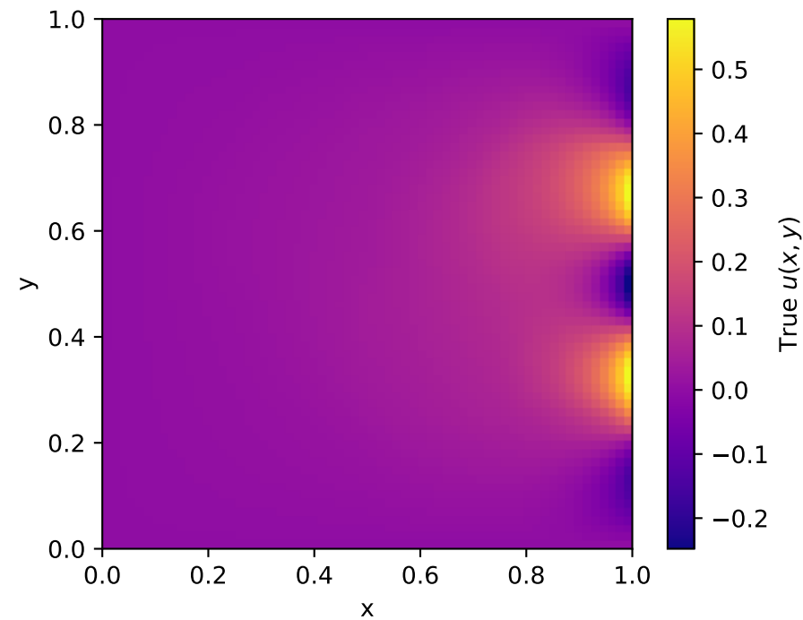
Induced Potential Field for k=15
