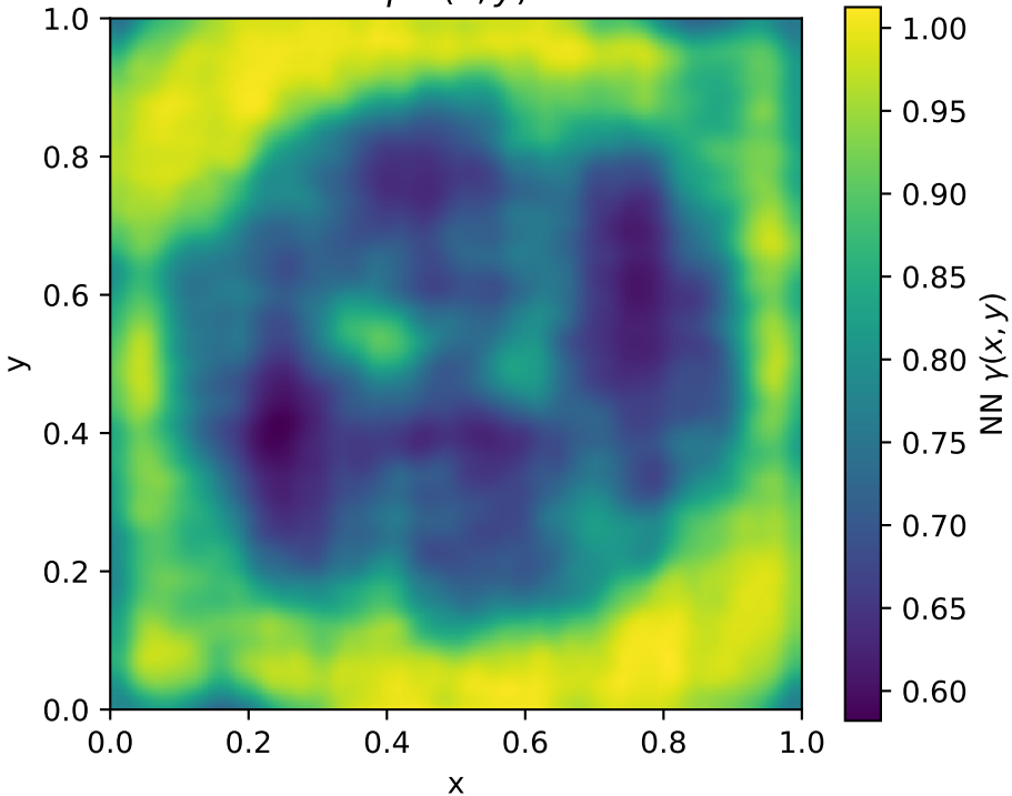
\gamma^{NN}(x, y)
