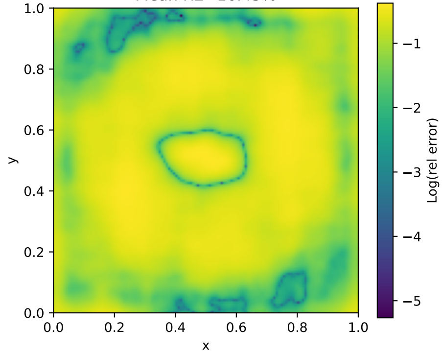
Mean RE=16.45%
