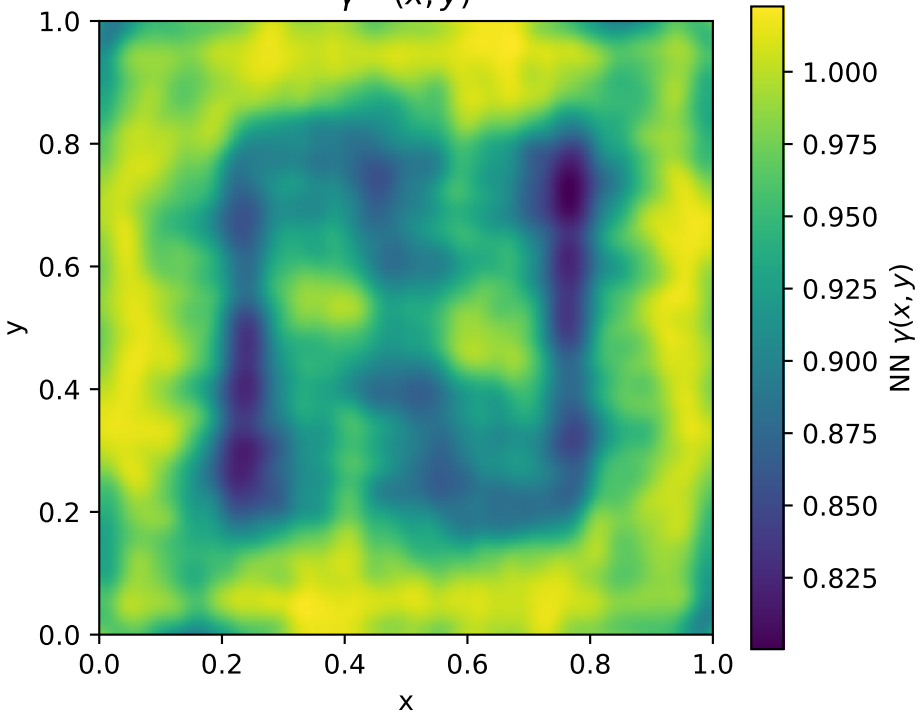
\gamma^{NN}(x, y)
