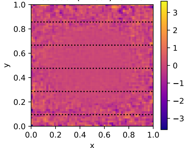
PDE Residual (Linear) for BC k=10
