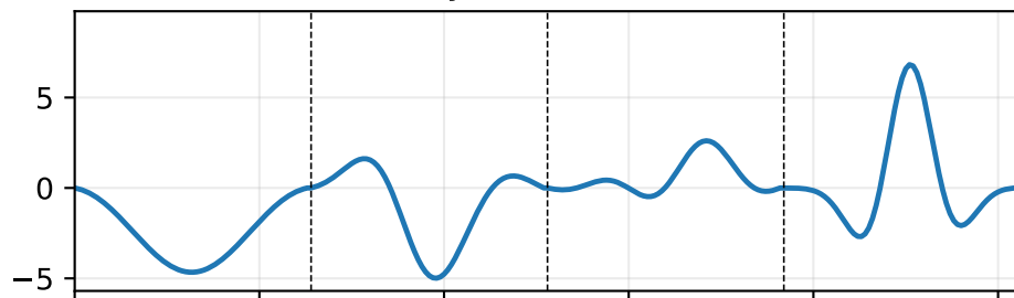
Boundary condition k = 84
