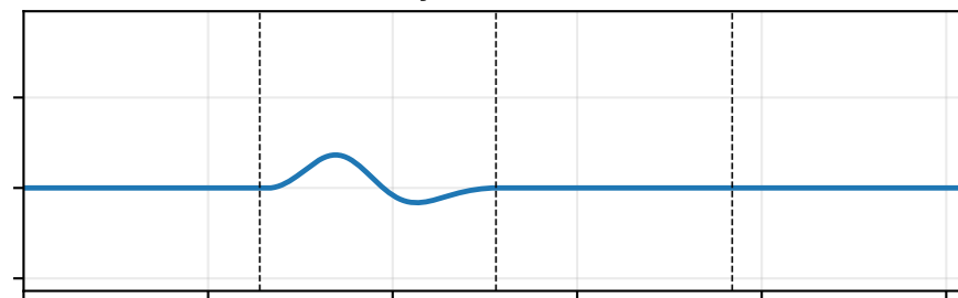
Boundary condition k = 14
