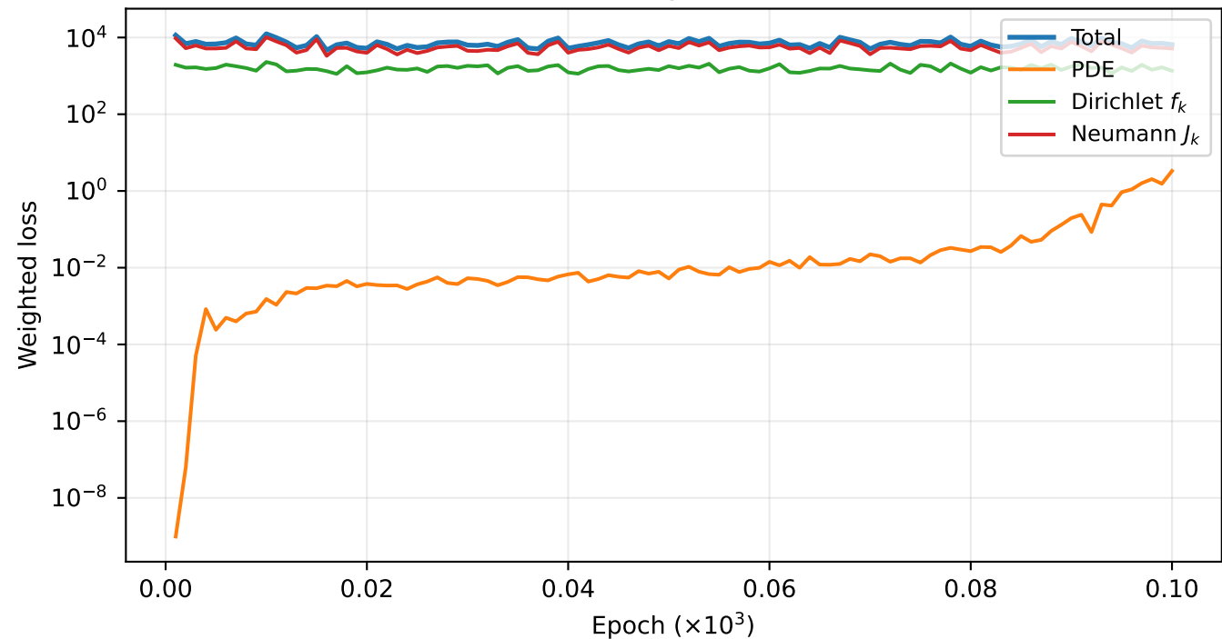
Training losses
