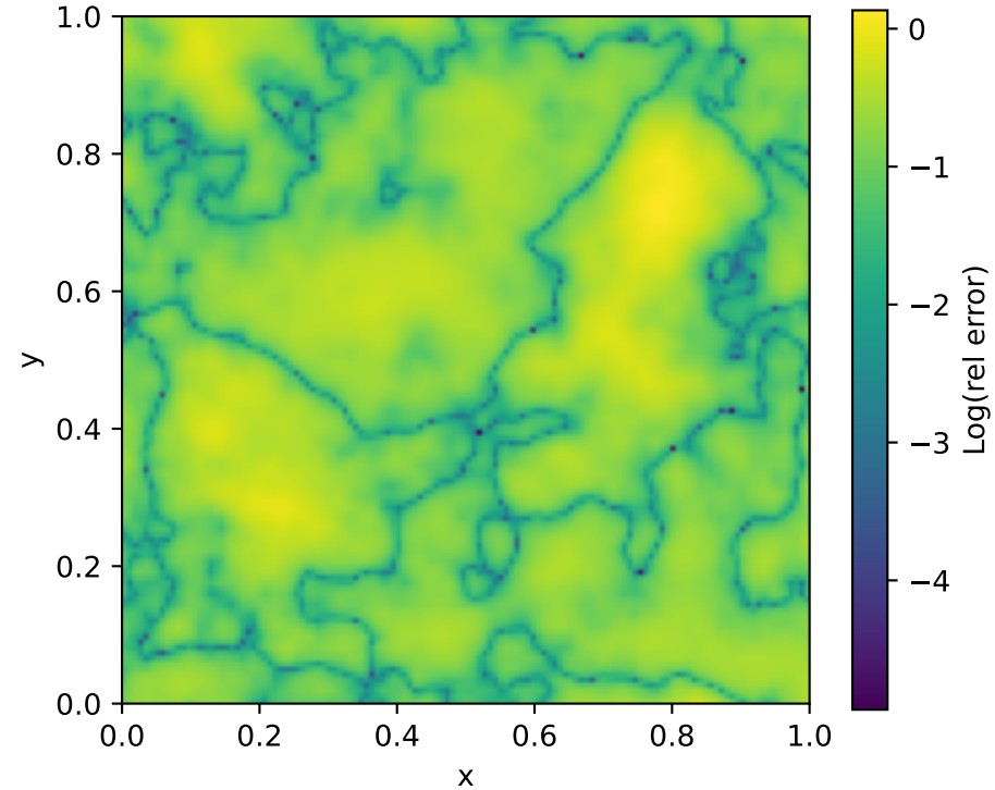
Mean RE=18.22%
