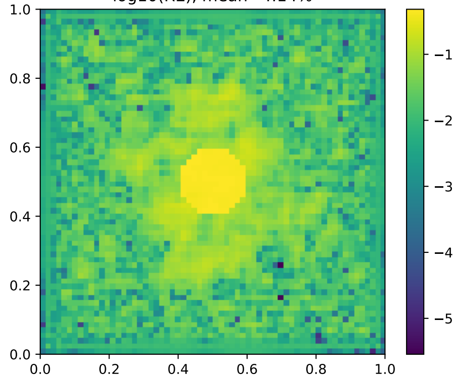
\log_{10}(\text{RE}), \text{mean}=4.14\%
