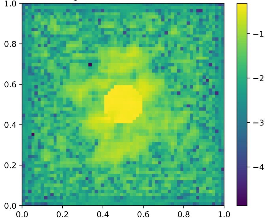
\log_{10}(\text{RE}) , mean=4.13%
