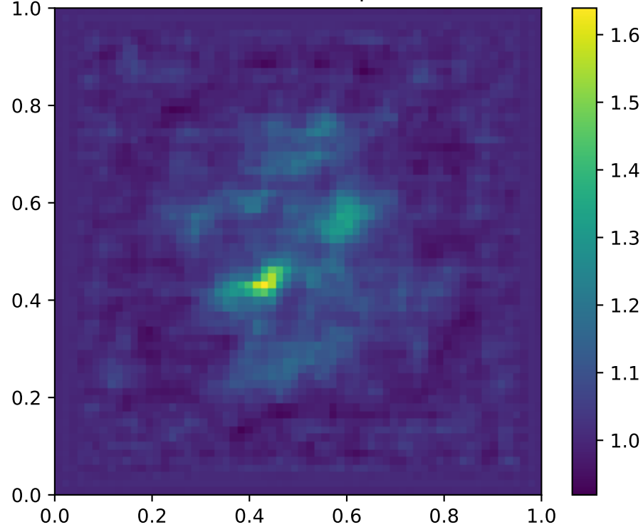
Recovered \gamma
