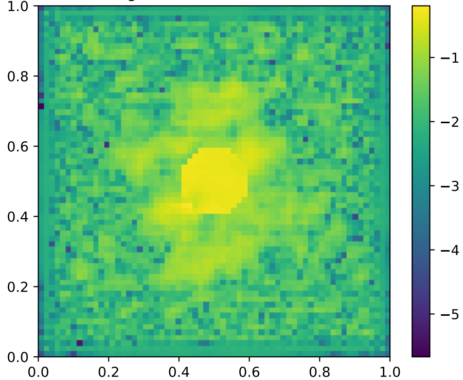
\log_{10}(\text{RE}) , mean=4.09%
