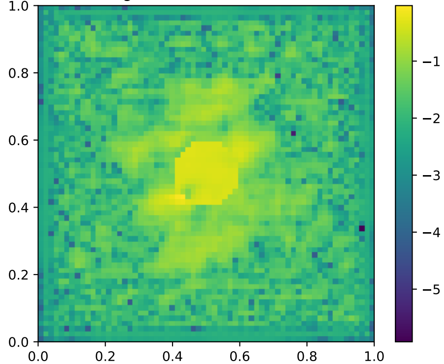
\log_{10}(\text{RE}) , mean=4.05%
