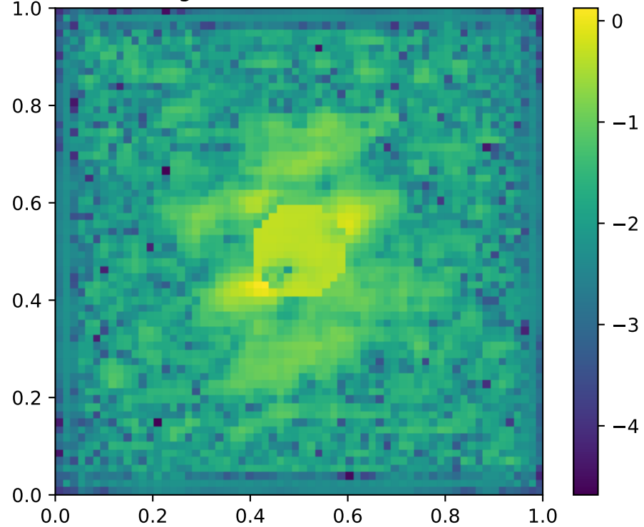
\log_{10}(\text{RE}) , mean=3.84%
