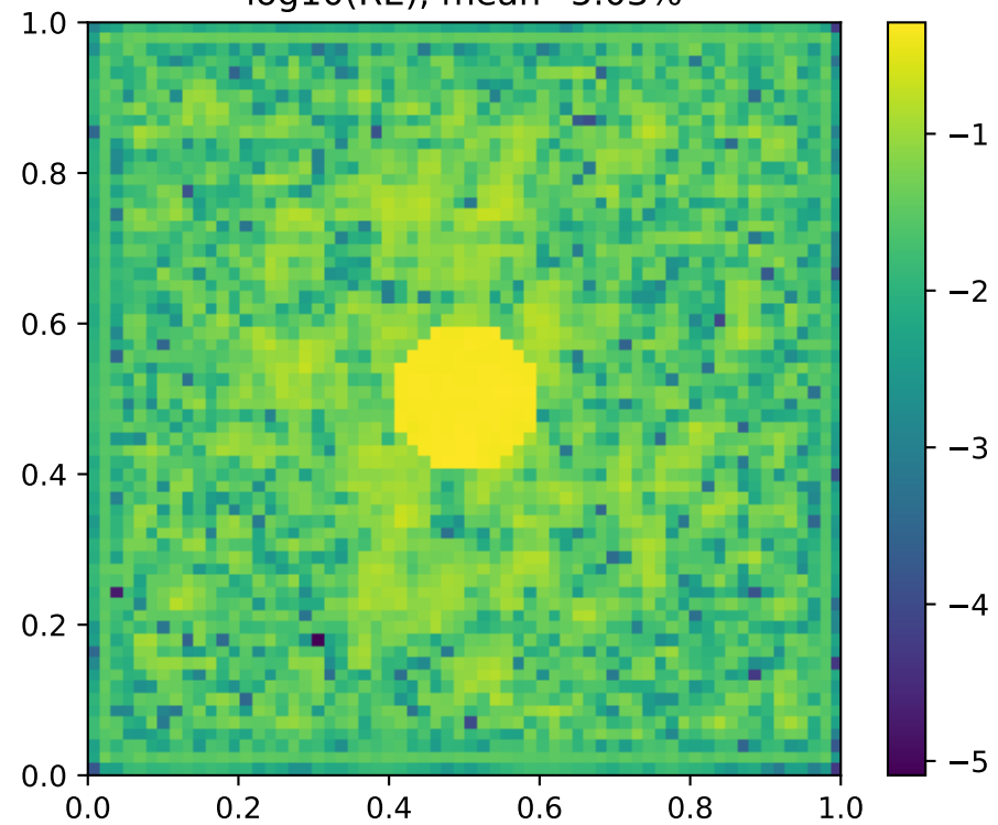
\log_{10}(\text{RE}) , mean=5.03%
