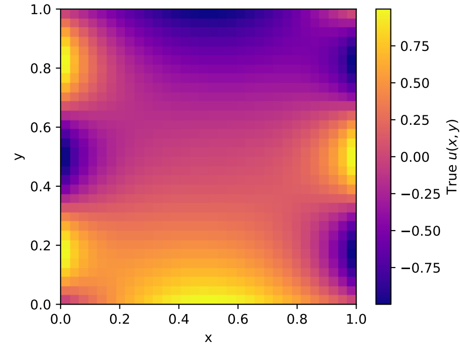
Induced Potential Field for k=23
