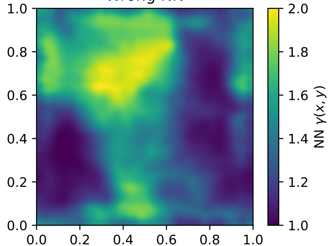
Wrong NN
