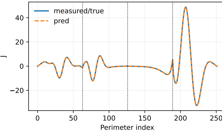
Current J_k ( k=40 )
