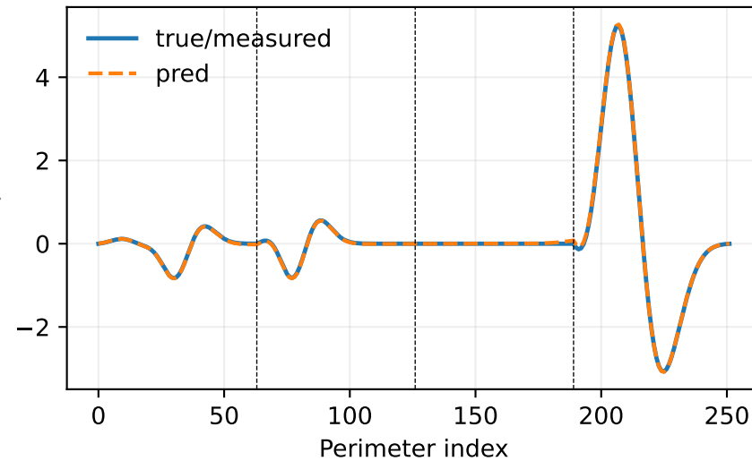
Dirichlet f_k ( k=40 )
