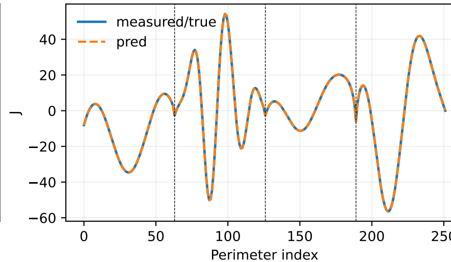
Current J_k ( k=20 )
