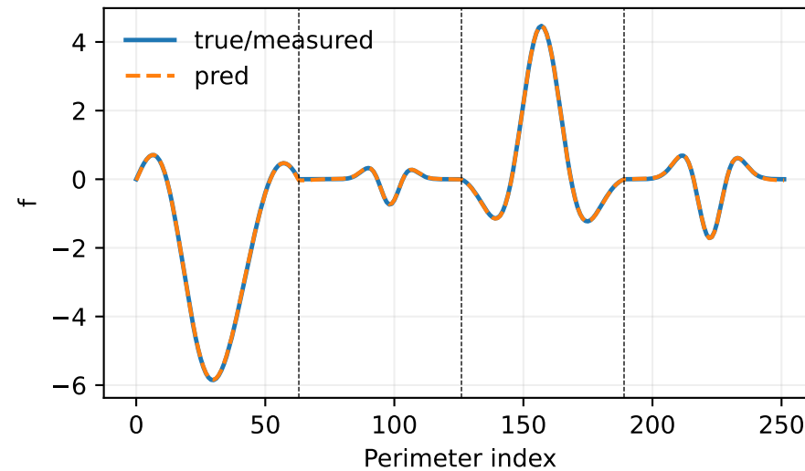
Dirichlet f_k ( k=40 )
