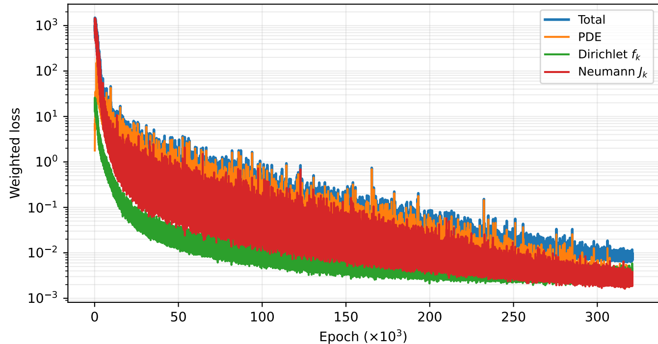
Training losses
