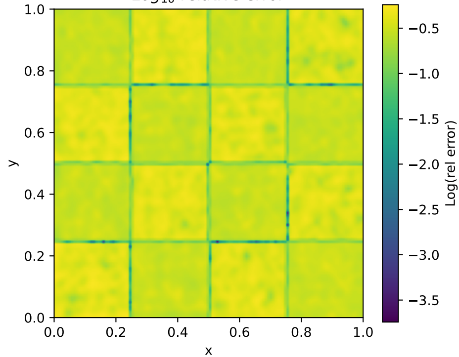
\text{Log}_{10} relative error
