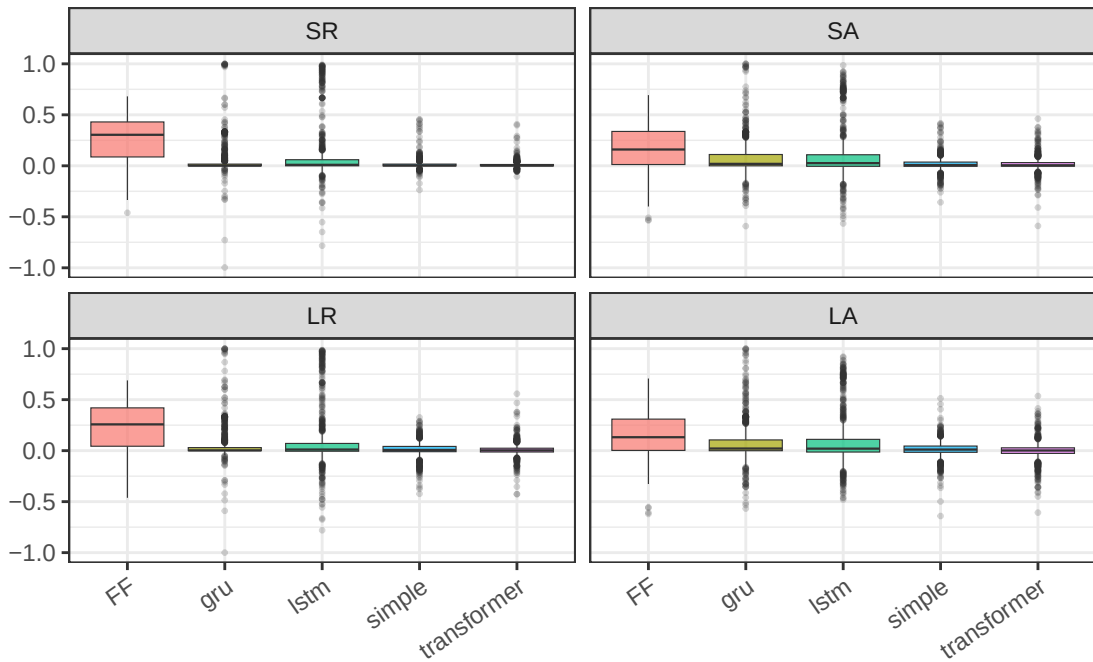
Difference in F1 Score from PS to OL by Model (Small train)
