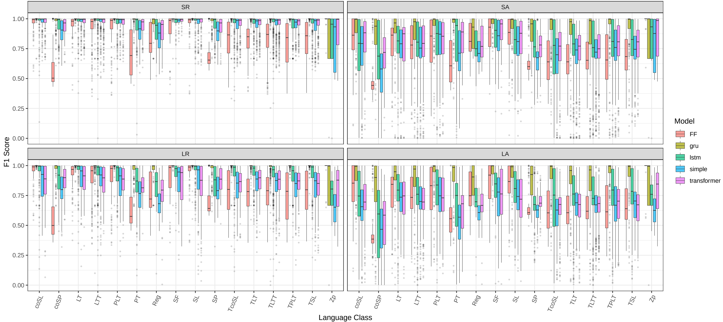
Average F1 by Language Class + Model on PlusShort
