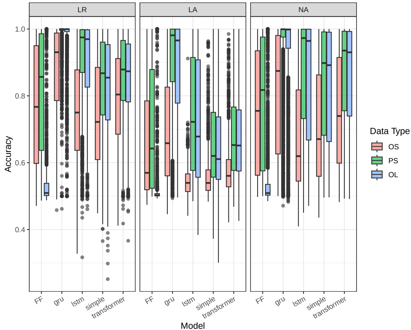
Average Accuracy by Data Type
