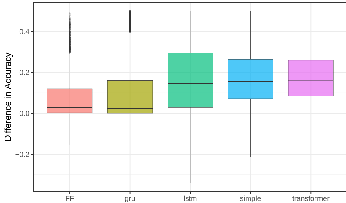
Difference in Accuracy between LR and LA Test Sets
