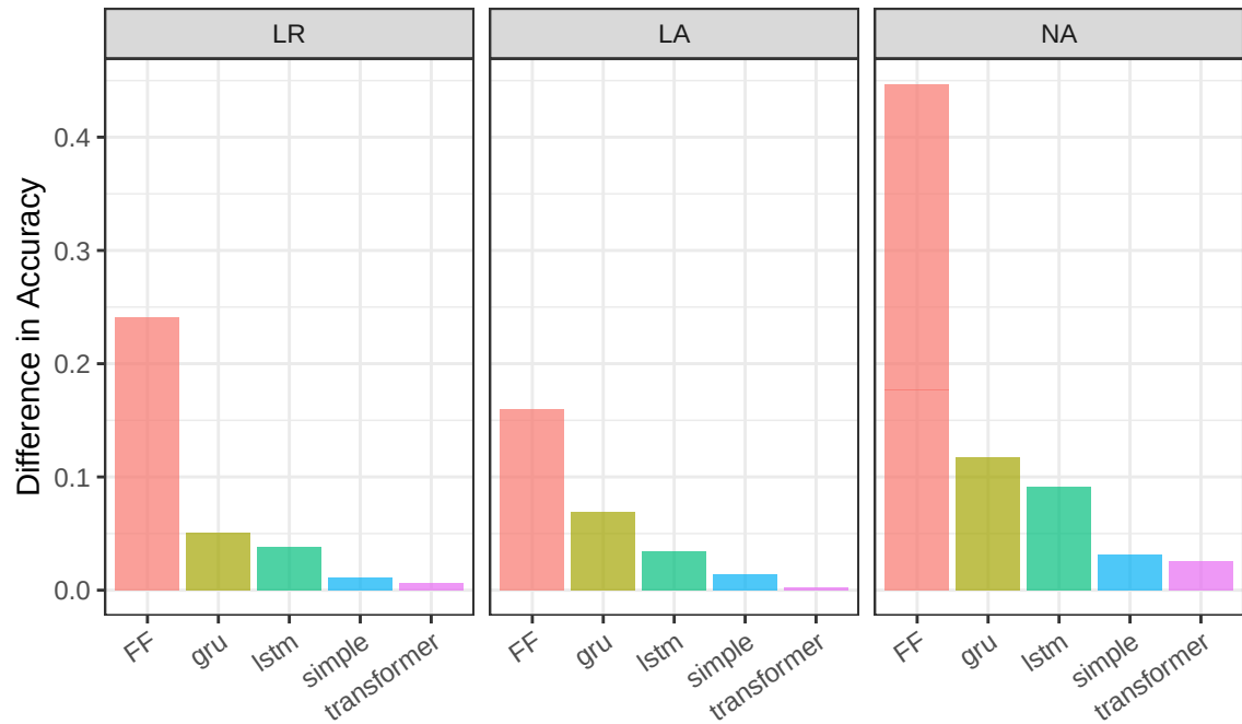
Difference in Acc from Small-PS to OI by Model
