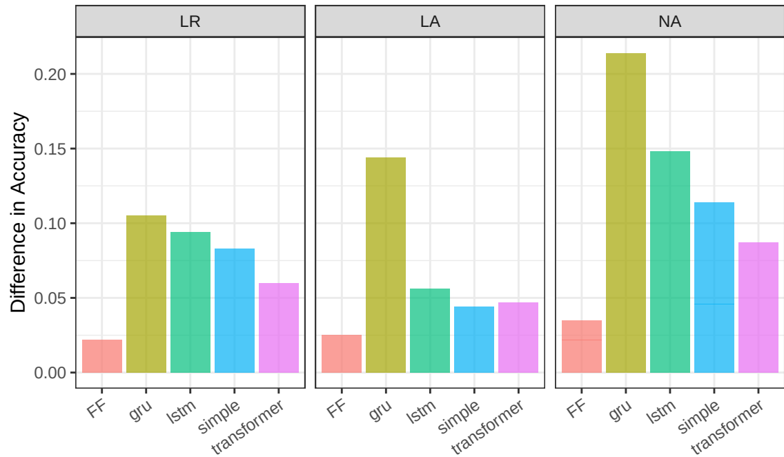
Difference in Acc from Small-PS to OS by Model
