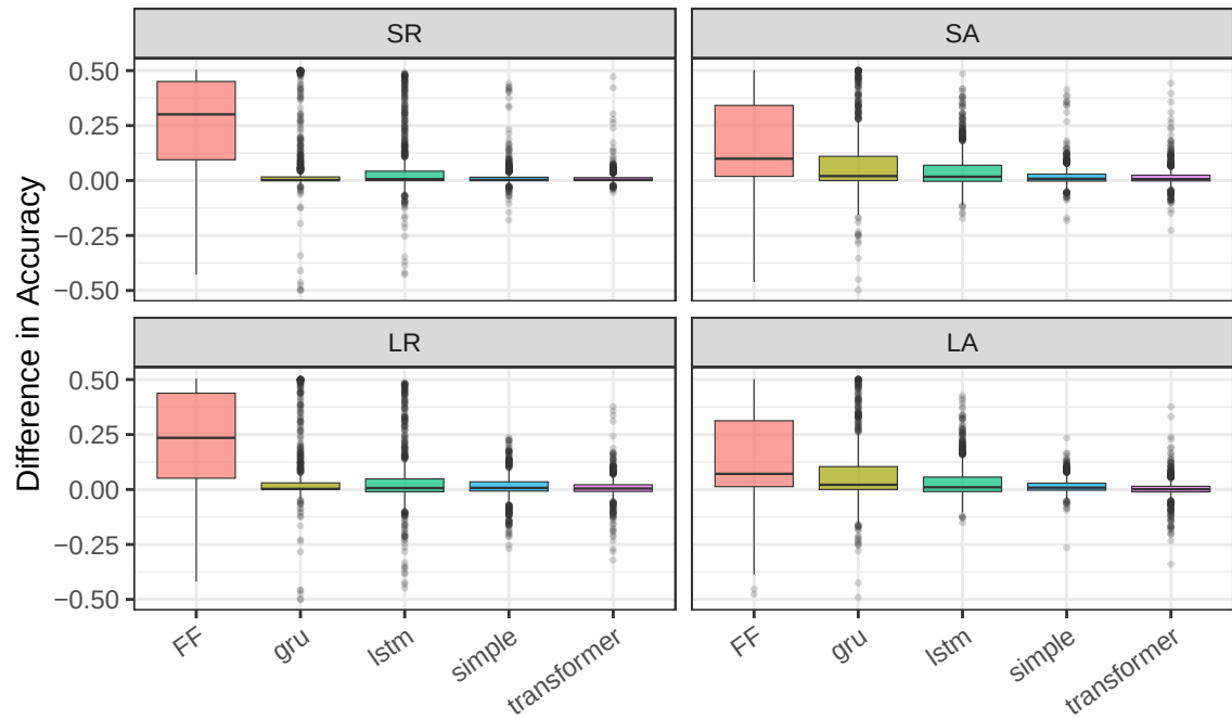
Difference in Accuracy from Small Plus Short to Only Short by Mode
