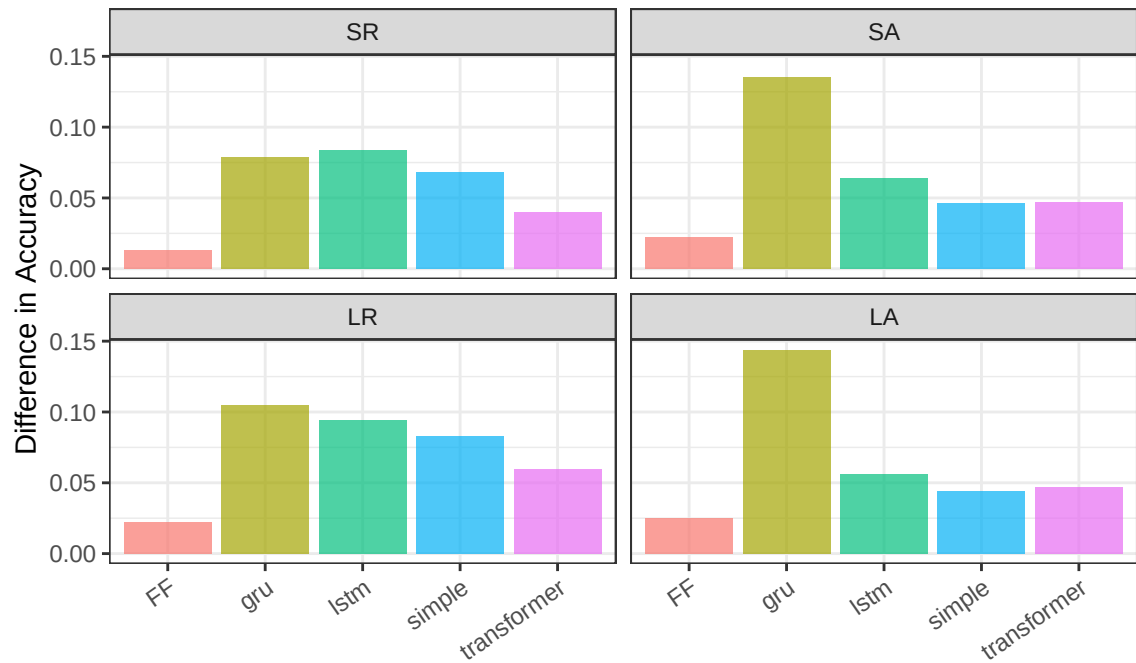
Difference in Accuracy from Small Plus Short to Only Short by Model
