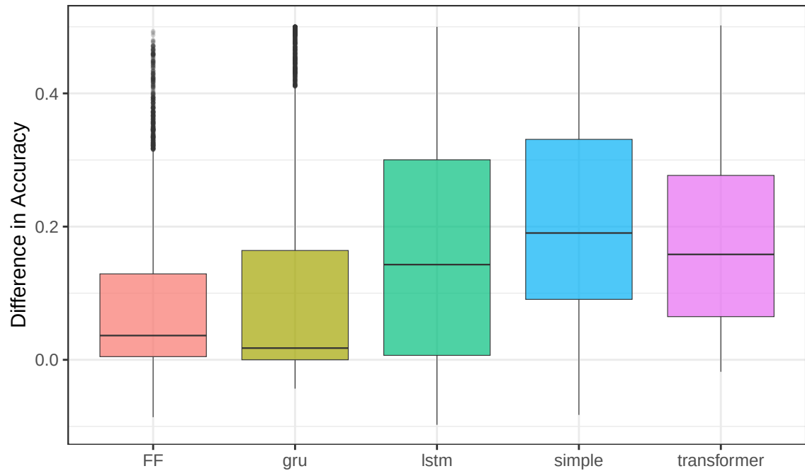
Difference in Accuracy between SR and SA Test Sets
