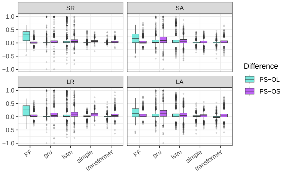
Difference in F1 Score Across Conditions by Model
