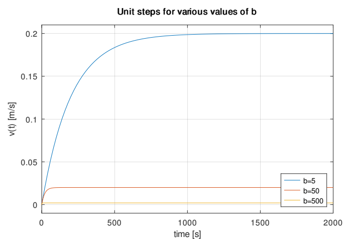
Figure 6: Unit step response of G_{V(s)} for b = 5 , b = 50 , and b = 500 .
