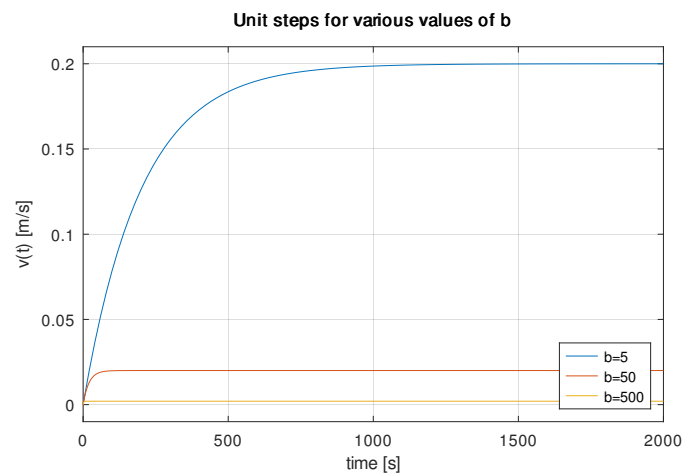
Figure 7: Unit step response of G_{V(s)} for b = 5 , b = 50 , and b = 500 .
