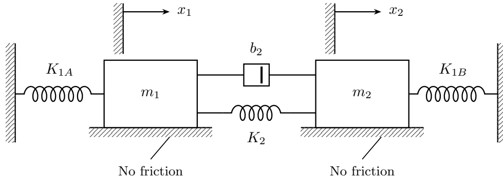
Figure 1: The two-mass system of Problem 1.B.
