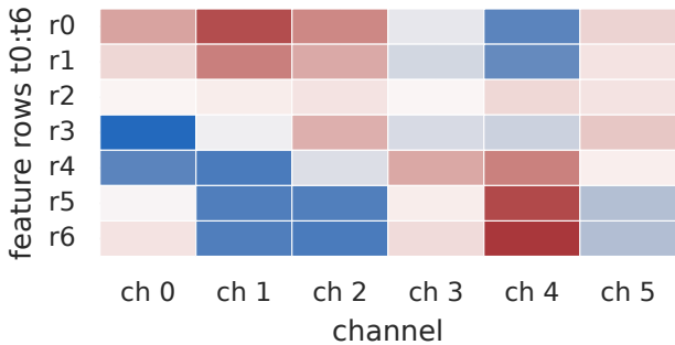
B. Design matrix slice X
