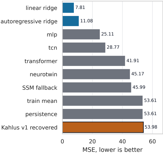
B. Masked reconstruction winner: linear ridge
