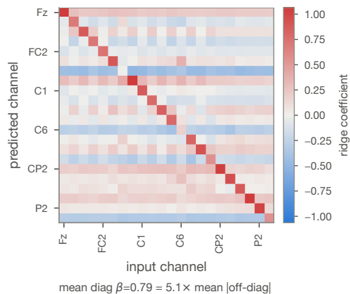
d Learned map is diagonally dominant
