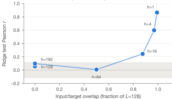
c Skill tracks overlap; zero overlap \Rightarrow noise floor
