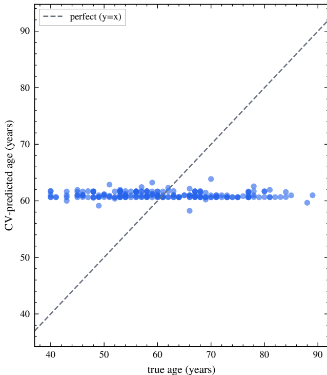
Bandpower brain-age: MAE 9.5 yr vs 9.4 baseline
