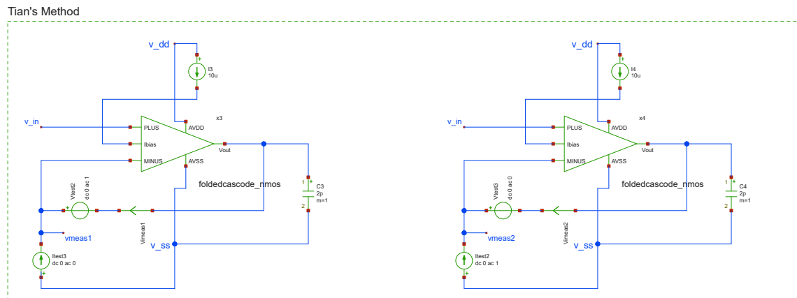
Figure 3.7.: Loop Gain Setup Tian
