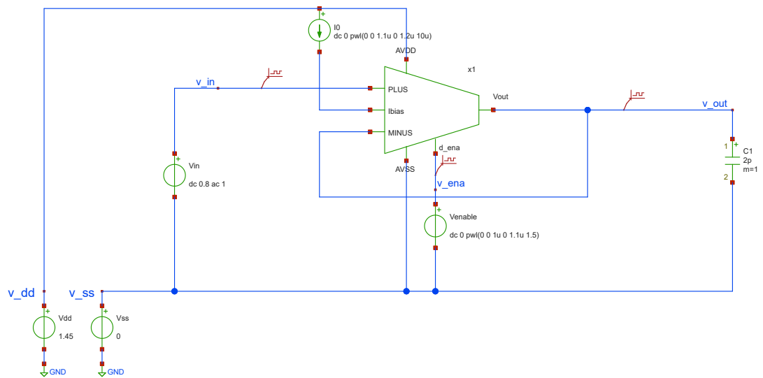
Figure 3.5.: Transient Analysis Setup
