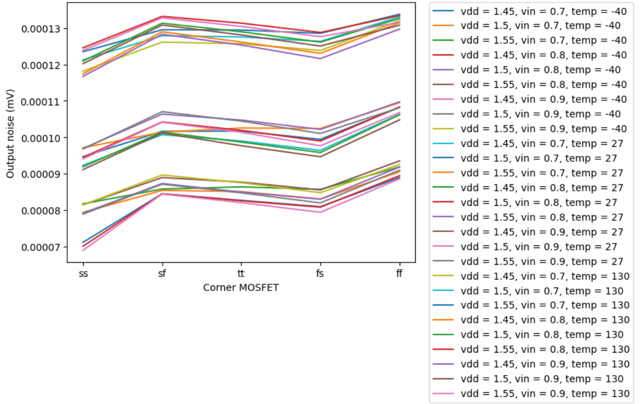
Figure 4.1.: noise_vs_corner
