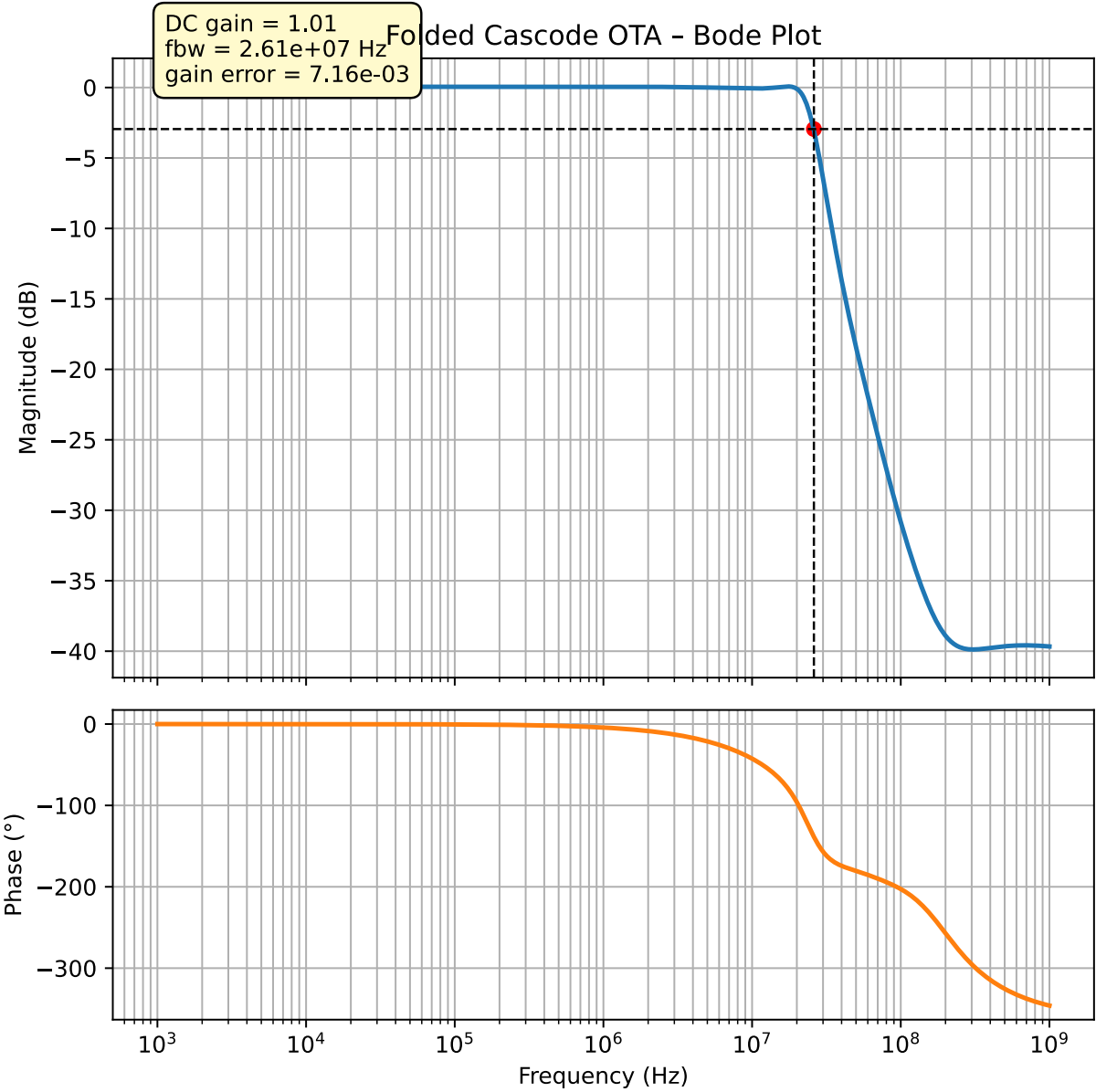
Figure 11.3.: Postlayout Results
